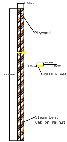
PLAN view of steam bent Oak or Walnut
